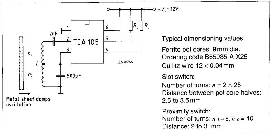
Circuit Diagram
